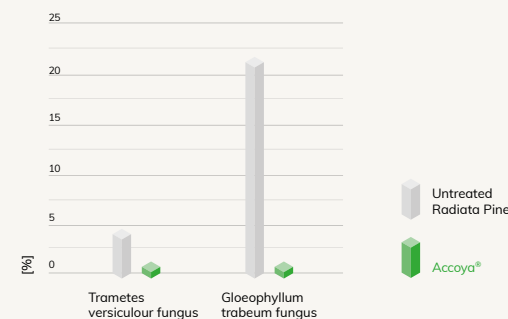
Weight loss in decay test
