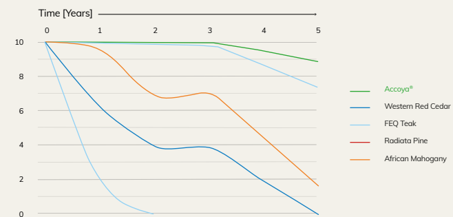
5 year Termite data (Gainesville FL, E7 Ground Contact)
